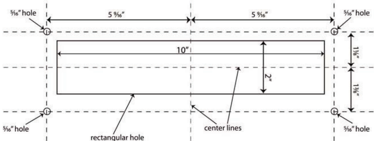
SMALL ( 11\frac{1}{16} " x 3\frac{1}{4} " ) Mail Slot Installation Dimensions (do not scale)
