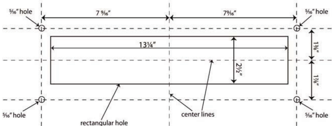
LARGE ( 15\frac{3}{4}" x 3\frac{15}{16}" ) Mail Slot Installation Dimensions (do not scale)
