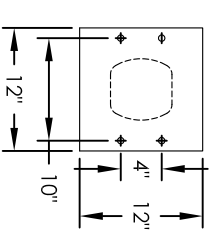
PEDESTAL DETAIL
