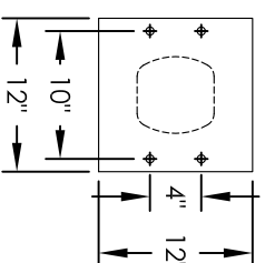
PEDESTAL DETAIL
