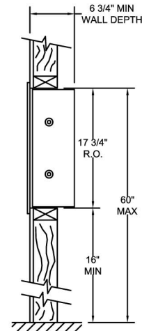
FINISHED FLOOR (RECESS MOUNT)
