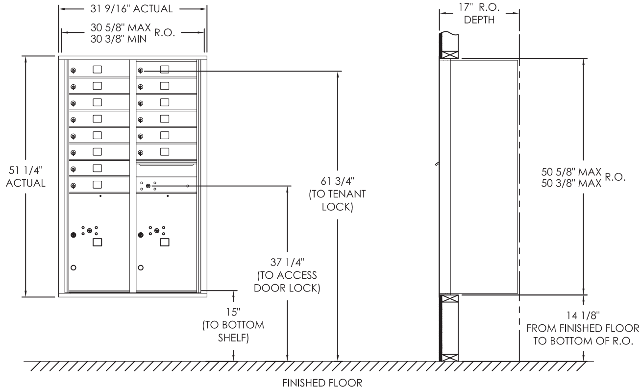
COMPARTMENT CHART
