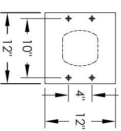
PEDESTAL DETAIL
