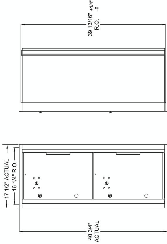
INSTALLATION EXAMPLE
